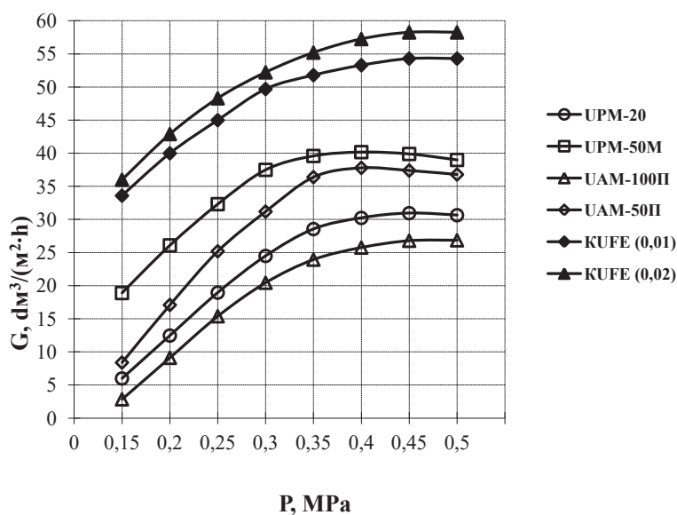
Fig. 5. Dependence of the permeability of UF membranes pressure (cheese necklace) at u = 3,0 \text{ m/s} ; t = 55 \text{ }^\circ\text{C} ; C = 12 \text{ \% СВ}
