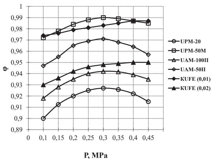
Fig. 7. Dependence of the selectivity of UF membranes on protein pressure (curd) at u = 3.0 \text{ m/s} ; t = 55^\circ\text{C} ; C = 12\% \text{ SV}
