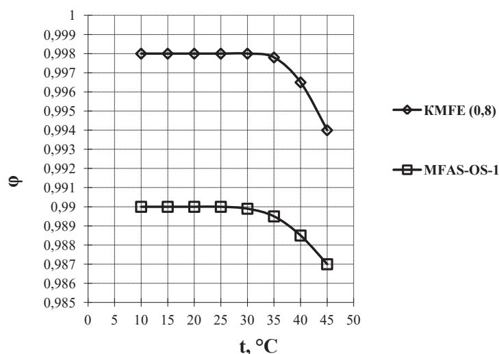
Fig. 10. Dependence of the selectivity of MF membranes on temperature (skimmed milk) at u = 4.5 m / s; P = 0.25 MPa; C = 8.5 % SV
