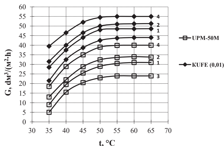
Fig. 9. Dependence of permeability of UF membranes on temperature (curd) at u = 3.0 m / s; P = 0.35 MPa. 1 – C = 17\% SV; 2 – C = 15\% SV; 3 – C = 20\% SV; 4 – C = 12\% SV
