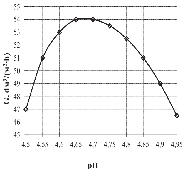
Fig. 12. Dependence of the permeability of UF membranes from the active acidity of the curd Callee at u = 3.0 m / s; P = 0.35 MPa, t = 55 °C; C = 12\% SV, membrane KUFЕ (0.01)
