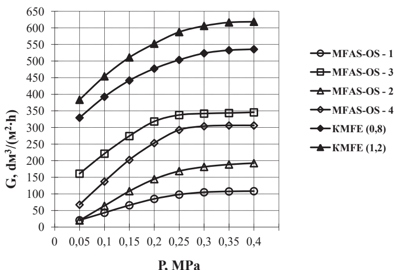
Fig. 4. Dependence of the permeability of MF membranes in the separation of skim milk from the pressure at u = 4.5 m/s; t = 35 °C; C = 8,5 % SV
