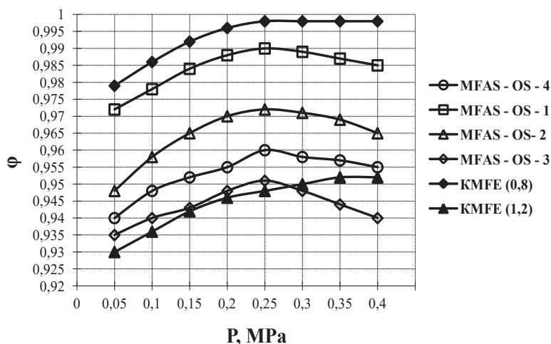
Fig. 6. Dependence of selectivity on microflora of MF membranes in the separation of skimmed milk from the pressure at u = 4,5 \text{ m/s} ; t = 35^\circ\text{C} ; C = 8,5\% \text{ SV}
