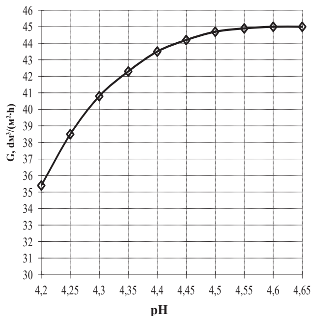
Fig. 13. Dependence of the permeability of UF membranes from UF active acidity of cheese at u = 3.0 m / s; P = 0.35 MPa, t = 55 °C; C = 15.0 % SV, membrane KUFЭ (0.01)
