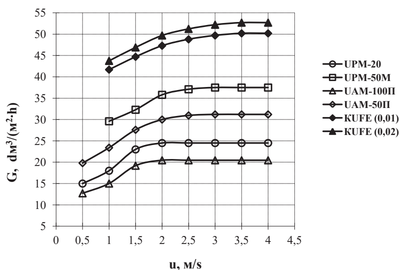
Fig. 3. Dependence of the permeability of UF membranes on the flow rate of curd over the membrane at P = 0.3 MPa; t = 55 °C; C = 12 % SV
