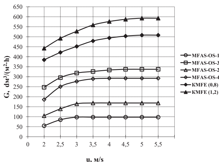
Fig. 2. Dependence of permeability of MF membranes on the flow rate of skimmed milk over the membrane at P = 0.25 MPa; t = 35 °C, C = 8.5 % SV
