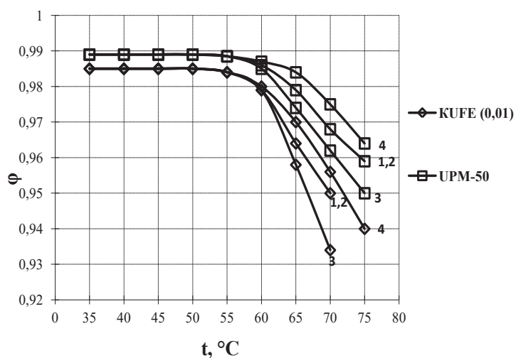
Fig. 11. Dependence of UF membrane selectivity on temperature (curd) at u = 3.0 m / s; P = 0.35 MPa. 1 - C = 17\% SV; 2 - C = 15\% SV; 3 - C = 20\% SV; 4 - C = 12\% SV
