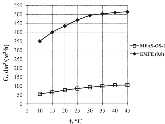
Fig. 8. Dependence of permeability of MF membranes on temperature (skimmed milk) at u = 4.5 m / s; P = 0.25 MPa; C = 8.5 % SV
