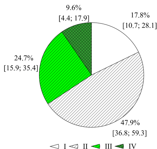
Fig. 5. Distribution of groundwater in the Sosnovskiy district of the Chelyabinsk region by quality category
