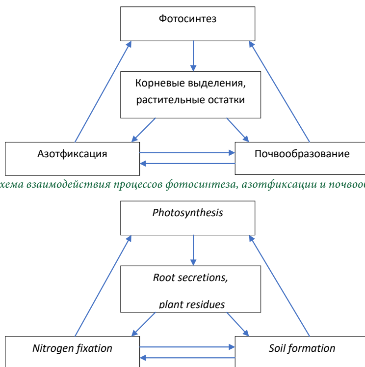
Fig. 1. Diagram of interaction of photosynthesis, nitrogen fixation and soil formation processes
